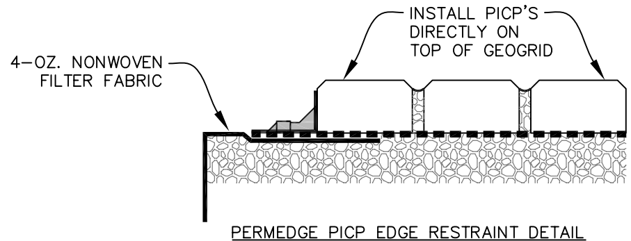
PERMEDGE PICP EDGE RESTRAINT DETAIL
