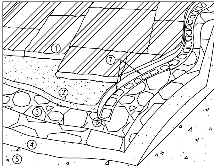
TYPICAL SEGMENTAL PAVER INSTALLATION
