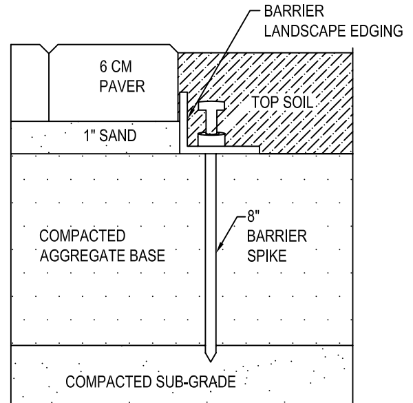
BARRIER INSTALLATION
